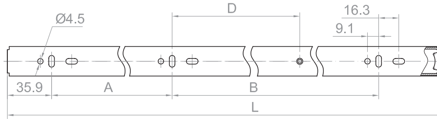
DRAWER MEMBER
